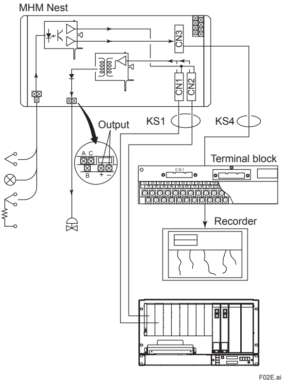
Figure 2. MHM-50 Nest Connection
