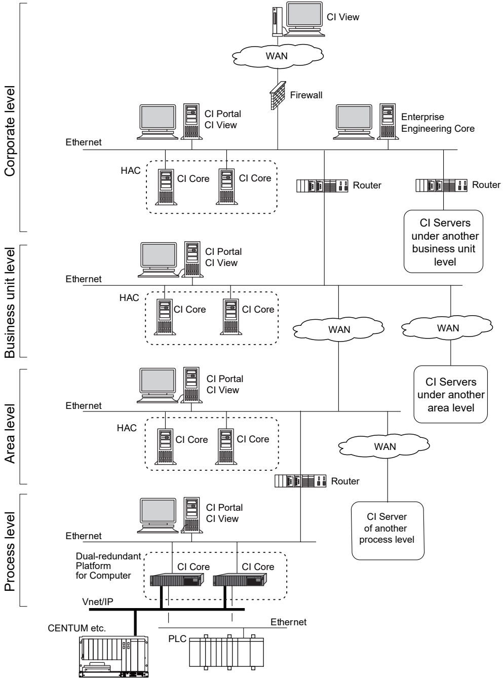
Figure Example of Enterprise Configuration
