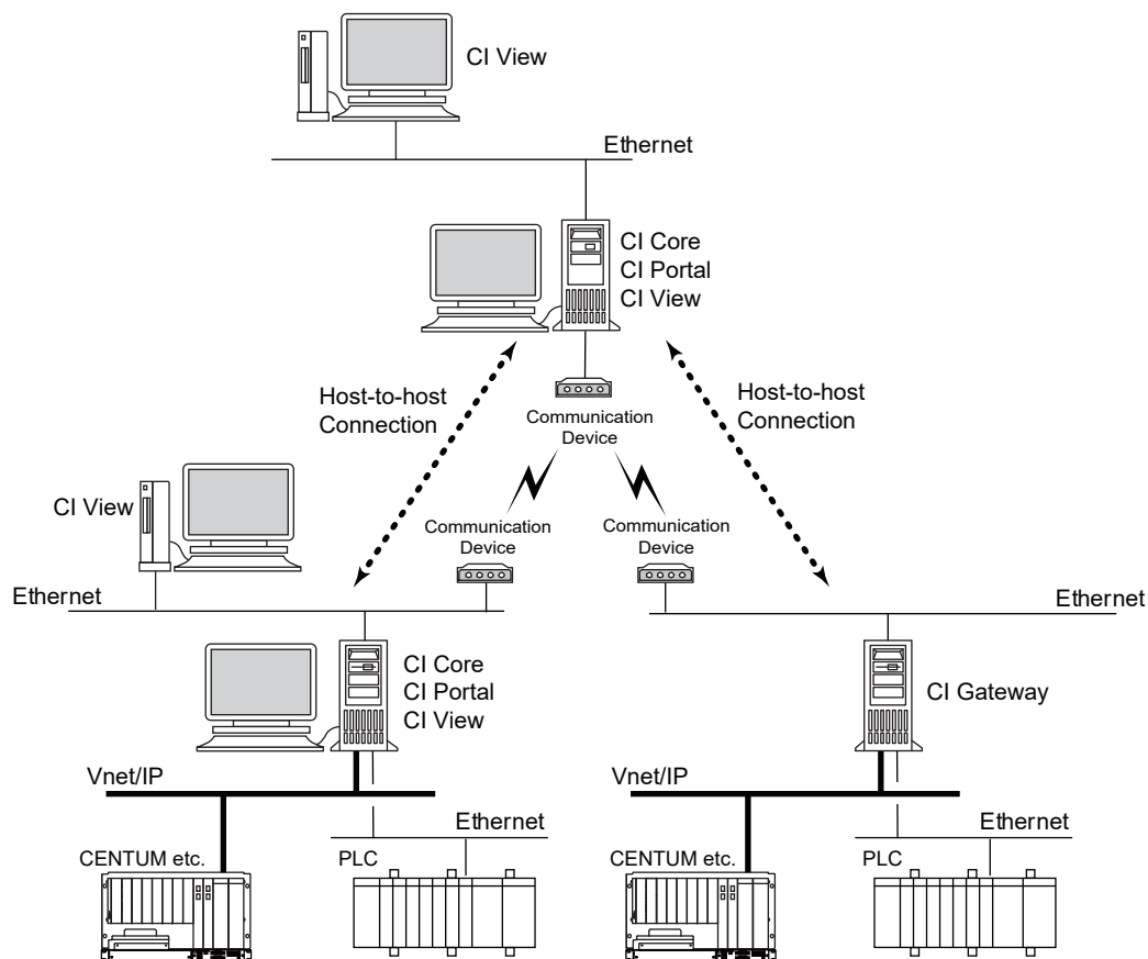
Figure Example of Host-to-host Connection Configuration
