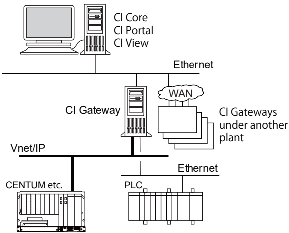
Figure Example of Gateway Configuration (CI Core)
