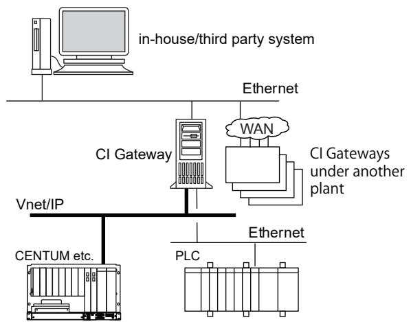
Figure Example of Gateway Configuration (in-house/third party system)
