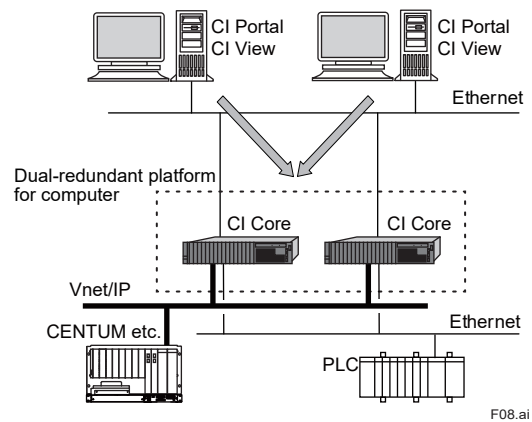
Figure Example of Dual-redundant Platform for Computer Configuration
